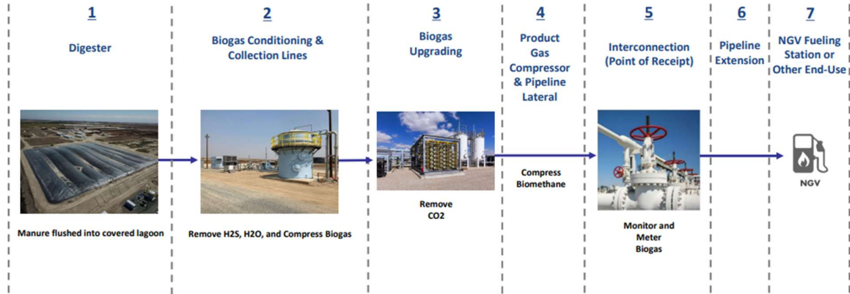
Figure 1: Process to Convert Dairy Biogas into R-CNG
