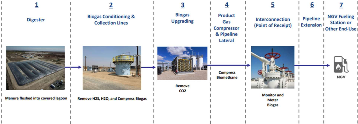
Figure 1: Process to Convert Dairy Biogas into R-CNG
