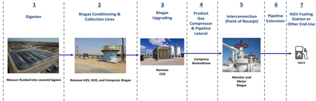
Figure 1: Process to Convert Dairy Biogas into R-CNG
