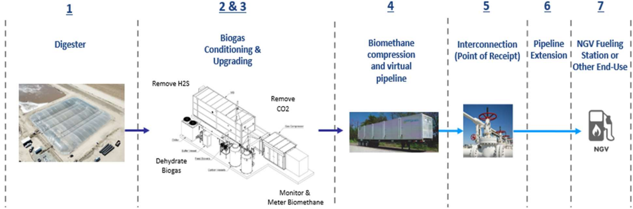
Figure 1: Biogas Processing
